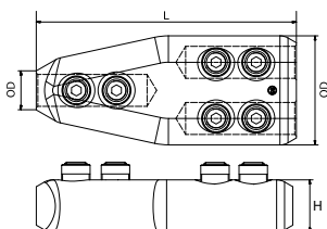
Branch Connector
