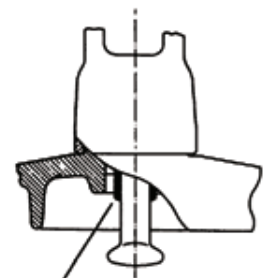
Corrosion prevention ring
